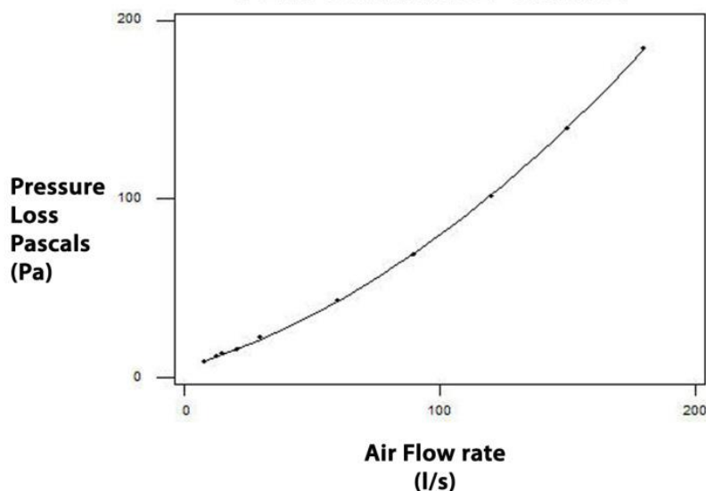
150mm 2m Round Pipe
